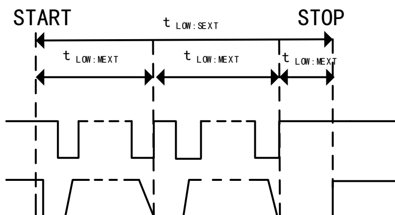
Figure 104 t_{\text{LOW:SEXT}} and t_{\text{LOW:MEXT}} Time
