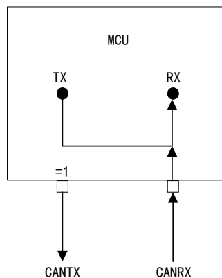
Figure 122 CAN Works in Silent Mode
