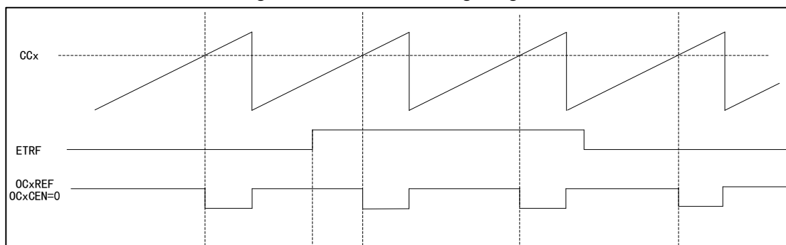
Figure 80 OCxREF Timing Diagram
