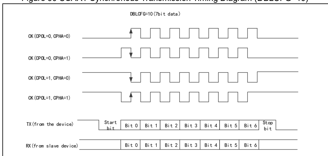
Figure 90 USART Synchronous Transmission Timing Diagram (DBLCFG=10)
