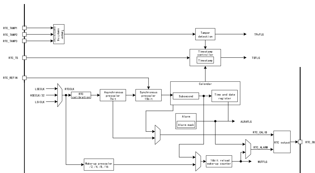
Figure 86 RTC Structure Block Diagram
