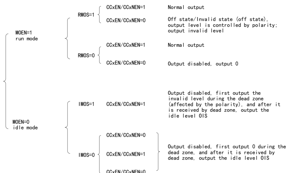
Figure 57 Register Structural Relationship Affecting Output Waveform
