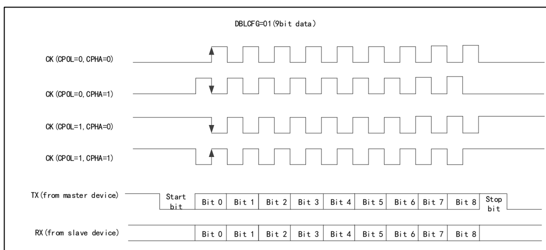
Figure 92 USART Synchronous Transmission Timing Diagram (DBLCFG=01)
