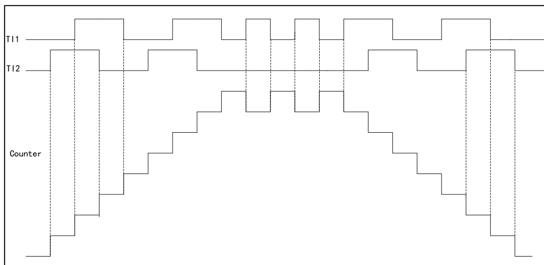
Figure 77 Counter Operation Example in Encoder Mode
