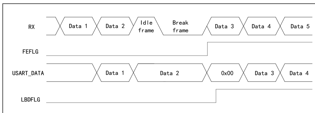
Figure 93 Break Frame Detection in Idle State
