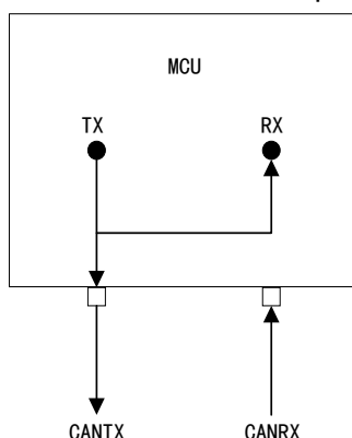
Figure 123 CAN Works in Loopback Mode
