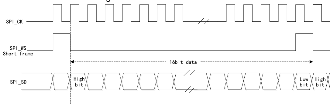
Figure 119 PCM Standard Waveform
