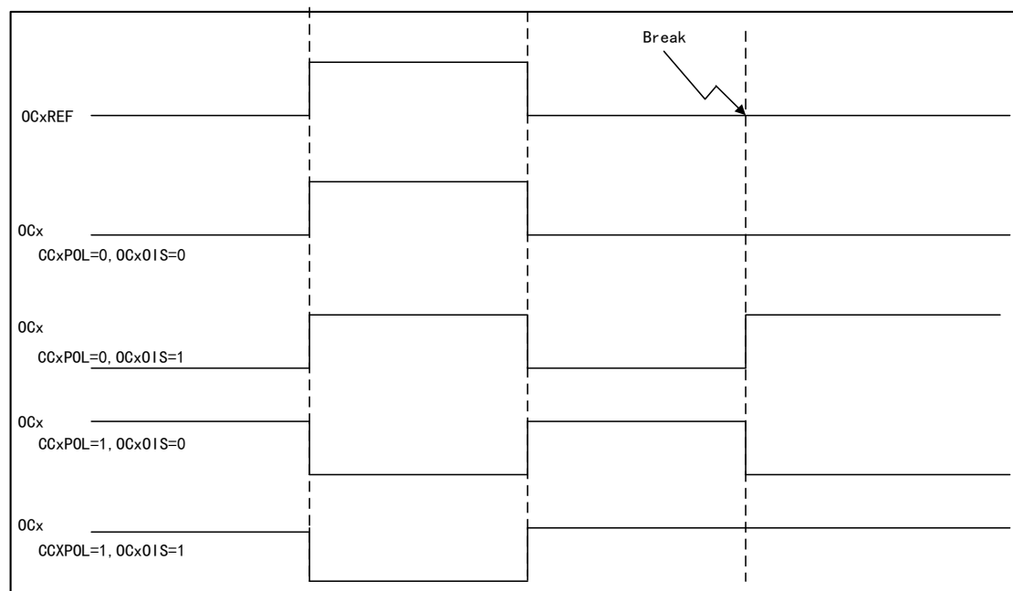
Figure 75 Breaking Event Timing Diagram
