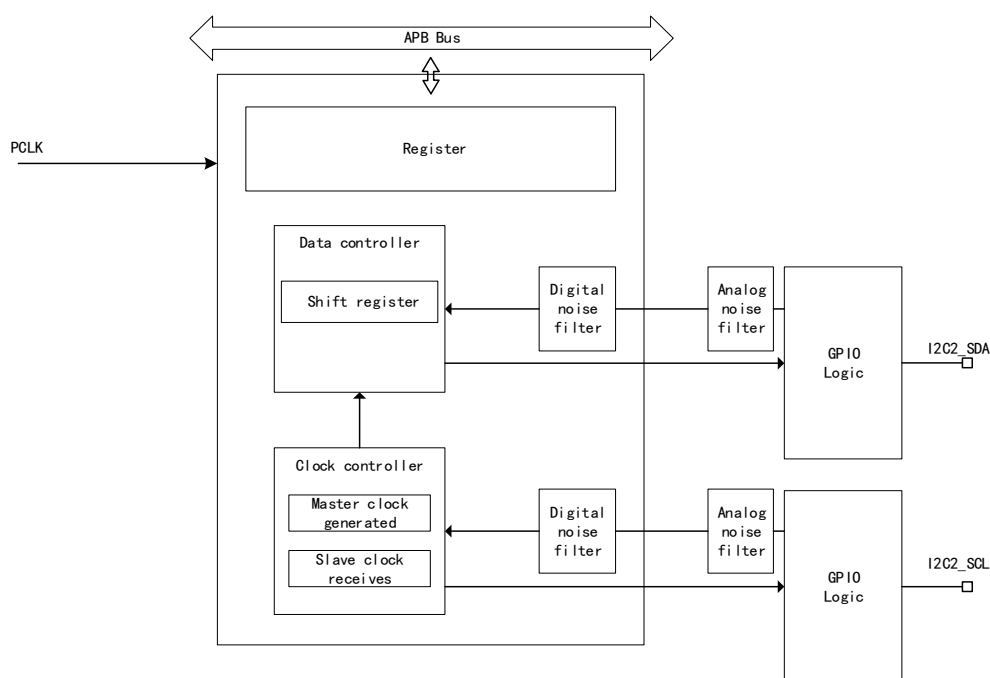
Figure 100 I2C2 Function Structure Diagram
