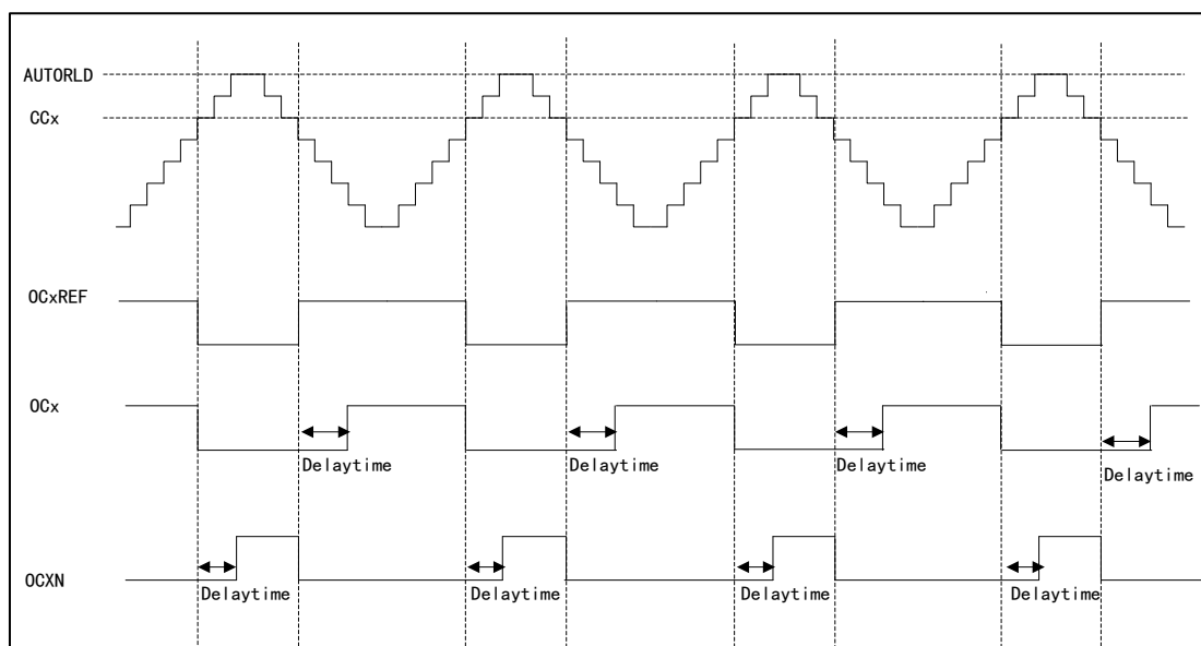
Figure 59 Complementary Output of Insertion with Dead-time
