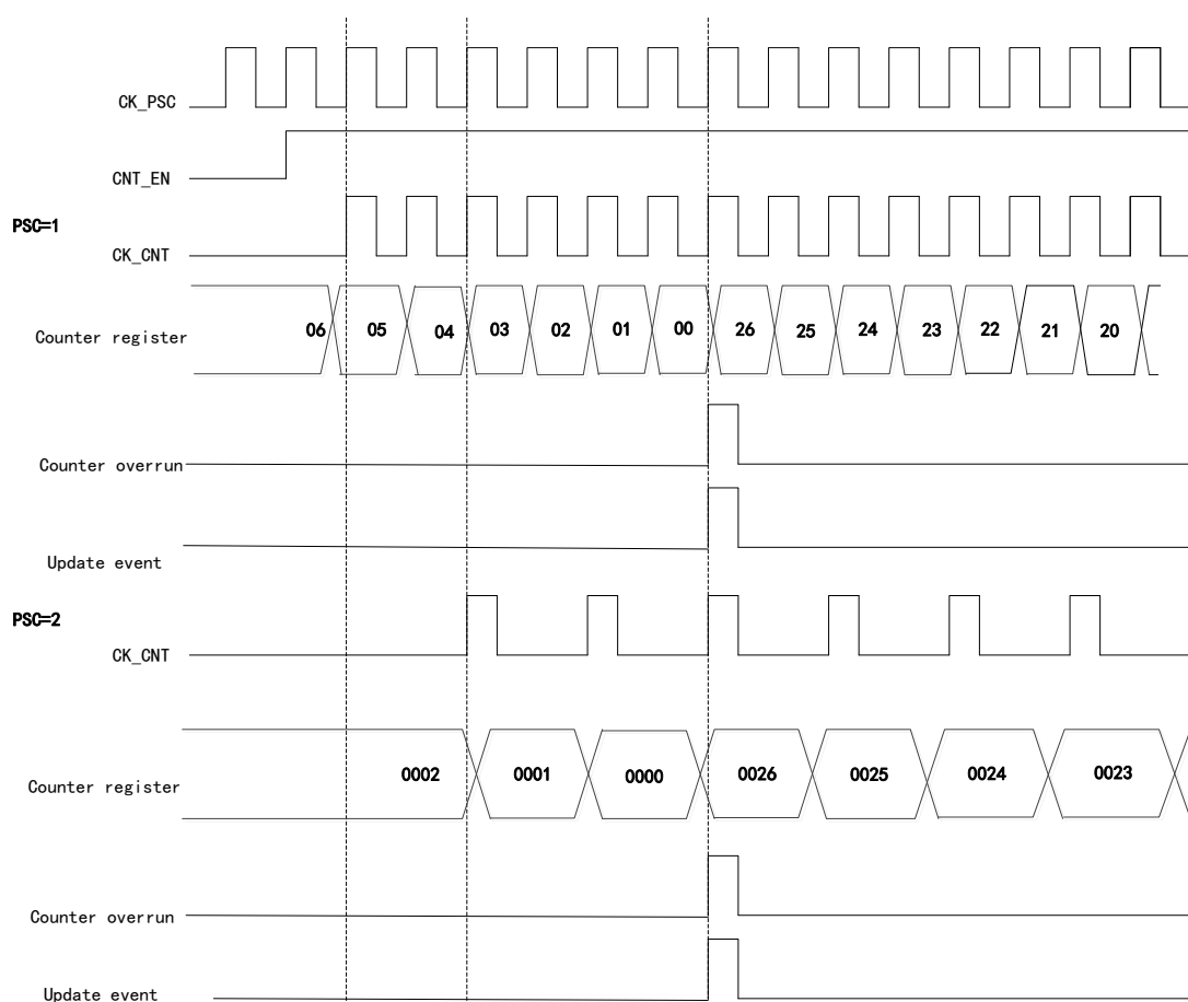
Figure 63 Timing Diagram when Division Factor is 1 or 2 in Count-down Mode
