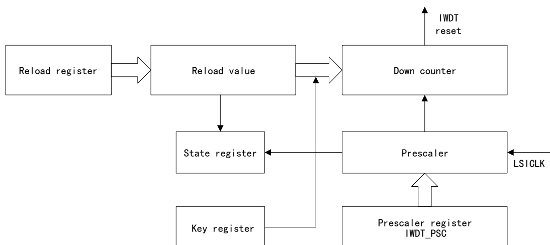
Figure 83 Independent Watchdog Block Diagram
