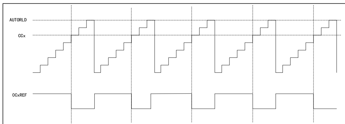
Figure 66 PWM1 Count-up Mode Timing Diagram
