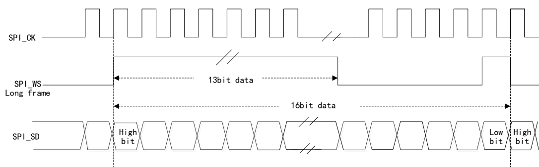
Figure 118 PCM Standard Waveform
